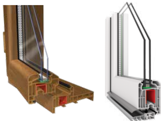
FRENCH FRAME PROFILE ALUMINIUM SILL SYSTEM
