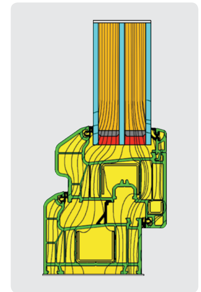
WINDOW HEAT FLOW DIAGRAM UF: 1,02 W/M² °K UW: 0,94 W/M² °K
