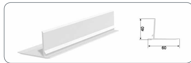
CLOSING PROFILE
