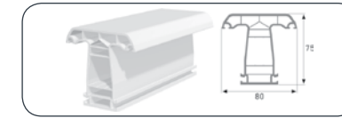
MULLION PROFILE
