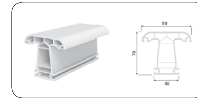
MULLION PROFILE
