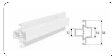
SLIDING SASH ADAPTING PROFILE
