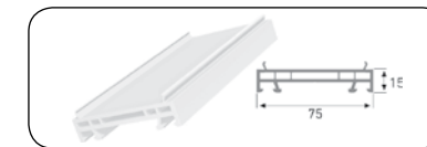
FRAME ELEVATION PROFILE (15 MM)
