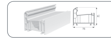
FRAME PROFILE
