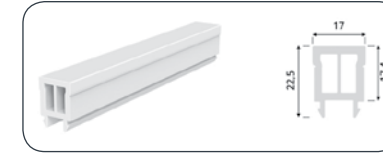
RAIL PASSING THE LOWER SIDE
