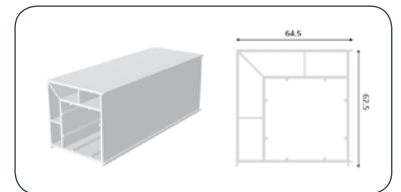
ANGLED POST BOX 90° PROFILE
