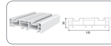
SLIDING FRAME PROFILE
