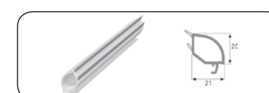
TRIPLE GLAZING BEAD PROFILE (32 MM)
