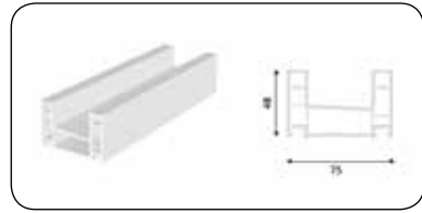
FRAME PROFILE
