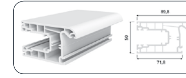
SLIDING SASH PROFILE
