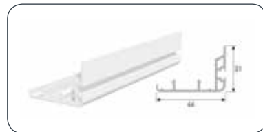
SLIDING SMALL SASH CLOSING PROFILE
