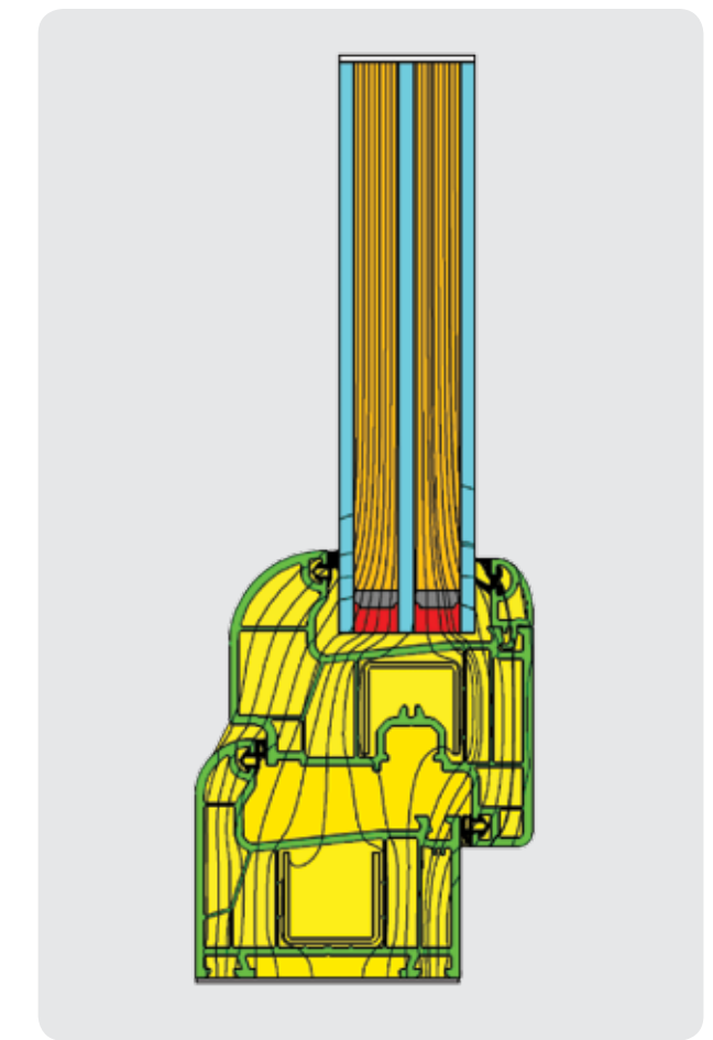
WINDOW HEAT FLOW DIAGRAM UF: 1,2 W/M² °K UW: 1,05 W/M² °K
