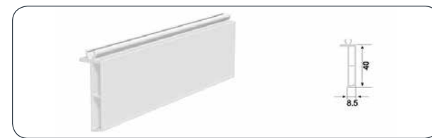
ZERO BASED LINING PROFILE
