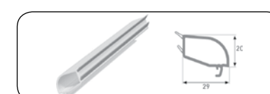
DOUBLE GLAZING BEAD PROFILE (24 MM)
