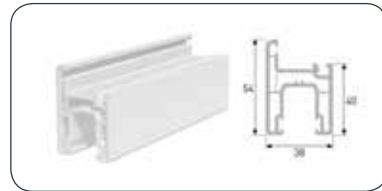
SLIDING SMALL SASH PROFILE
