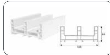
THREE TRACK SLIDING FRAME PROFILE
