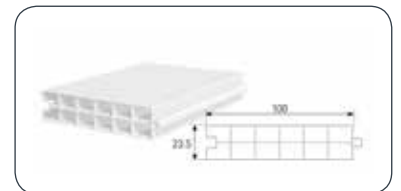
LAMBRI PROFILE (24X100 MM)
