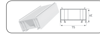
FRAME ELEVATION PROFILE (40 MM)
