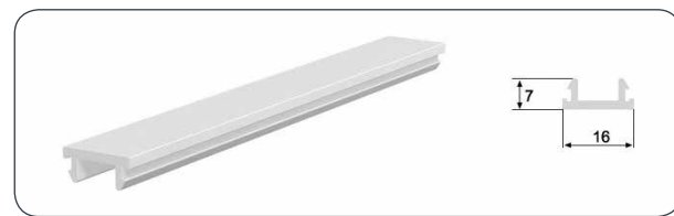
ESPAÑOLETTE CHANNEL CLOSING PROFILE
