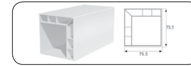
ANGLED POST BOX 90° PROFILE
