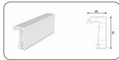
FIX PROFILE
