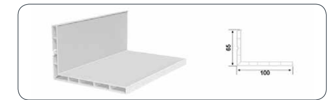
65X100 WINDOW LINING PROFILE
