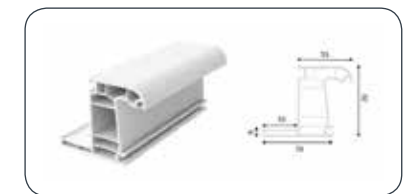
35 MM LINING FRAME PROFILE
