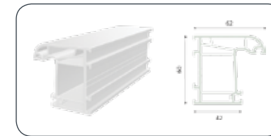
FRAME PROFILE
