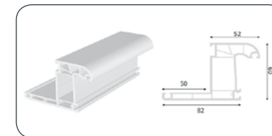
WIDE LINING FRAME
