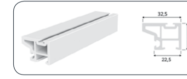
SASH CLAMP PROFILE
