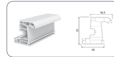
SASH PROFILE
