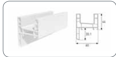
SLIDING FRAME PROFILE WITH LINING
