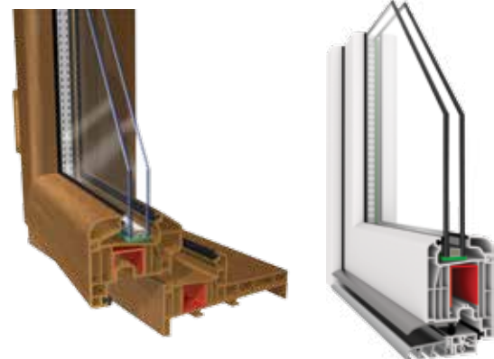
FRENCH FRAME PROFILE ALUMINIUM SILL SYSTEM
