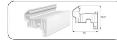
DRAINED SASH PROFILE
