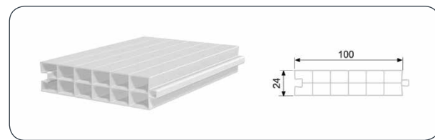
100X24 MM LAMBRI PROFILE
