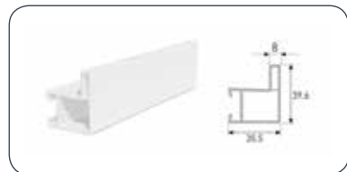
SLIDING FLY SWATTER FRAME PROFILE
