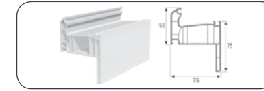
LINING FRAME PROFILE
