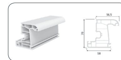
SASH PROFILE
