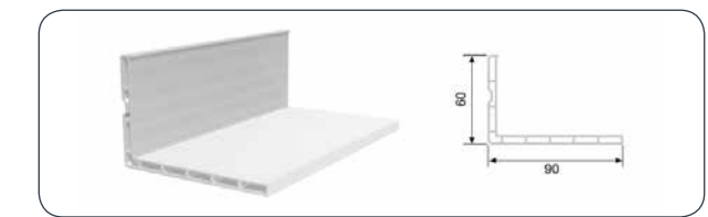
60X90 MM WINDOW LINING PROFILE
