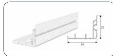
SLIDING BIG SASH CLOSING PROFILE
