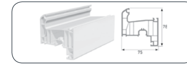
SASH PROFILE
