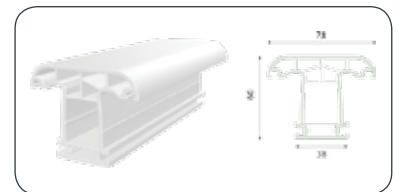
MULLION PROFILE
