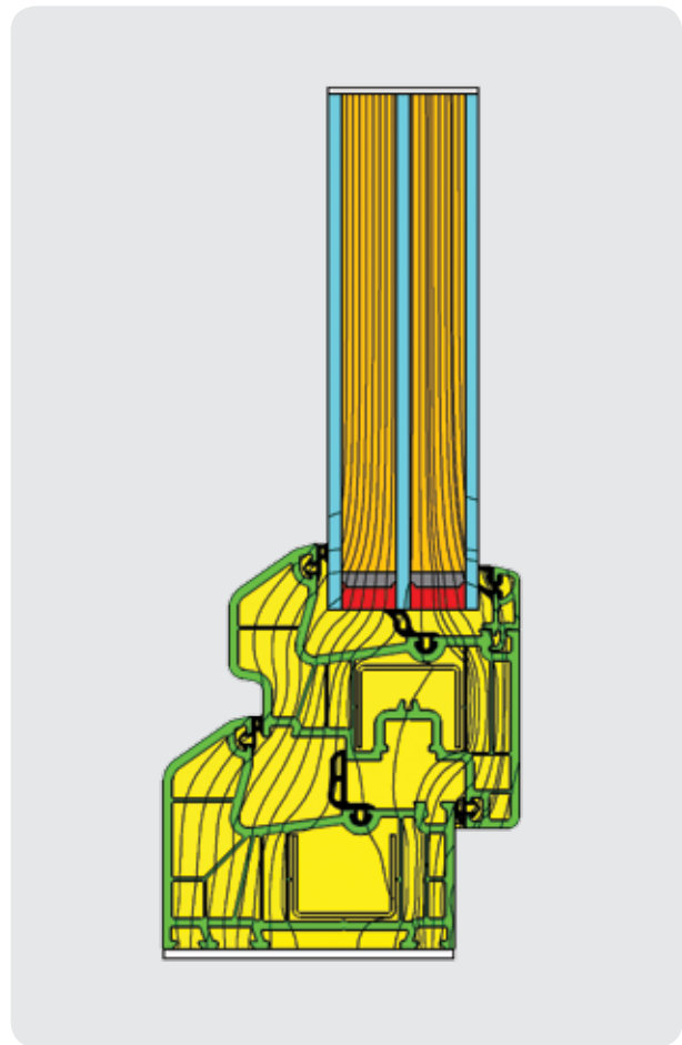
HEAT FLOW DIAGRAM
