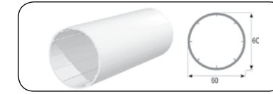
ANGLED POST ADAPTING PIPE PROFILE
