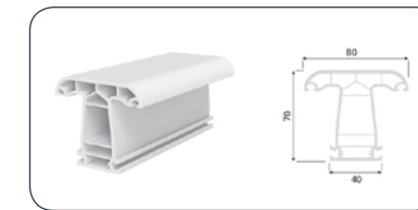
MULLION PROFILE
